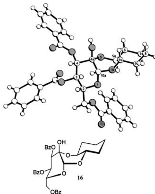
Figure 3. X-ray structure of the cis-transoid-trans -interconnected tricycle 16 [13] resulting from reaction of ulosyl bromide 5 with ( S,S )-1,2-cyclohexanediol; the chair conformations of the pyran and cyclohexane rings are contrasted by the central dioxane ring in a distorted boat form; selected torsional angles: \text{O1}-\text{C10a}-\text{C4a}-\text{O4a} 176.6, \text{O1}-\text{C10a}-\text{C4a}-\text{O5} -63.4, \text{O5}-\text{C4a}-\text{C10a}-\text{O10} 55.7, \text{O5}-\text{C5a}-\text{C9a}-\text{O10} 61.5
