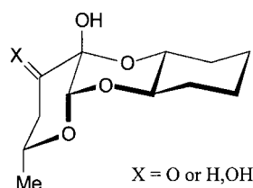
Figure 2. The linkage geometry in various cardiac glycosides and in the antibiotic spectinomycin is invariably cis-cisoid-trans [7]
