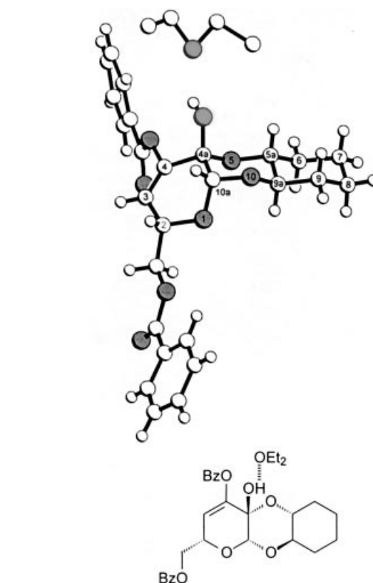
Figure 4. X-ray structure of the cis-cisoid-trans -fused 29 mono-etherate: due to the presence of a double bond, the pyran ring adopts the typical half-chair geometry versus nearly perfect chair conformations of the dioxane and cyclohexane parts. The acetalic 4a-OH and the pyranoid oxygen are in a trans -diaxial disposition ( \text{O1}-\text{C10a}-\text{C4a}-\text{O4a} : 164.8^\circ ) [16]
