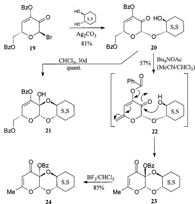
Scheme 5
