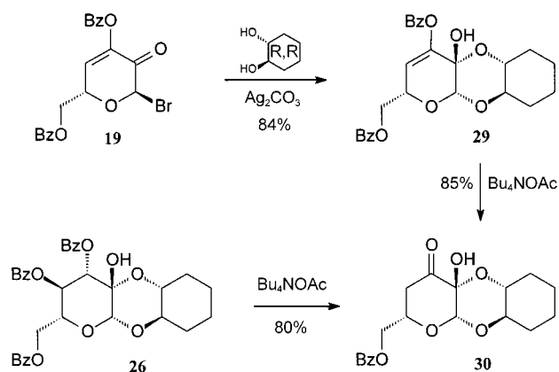
Scheme 7
