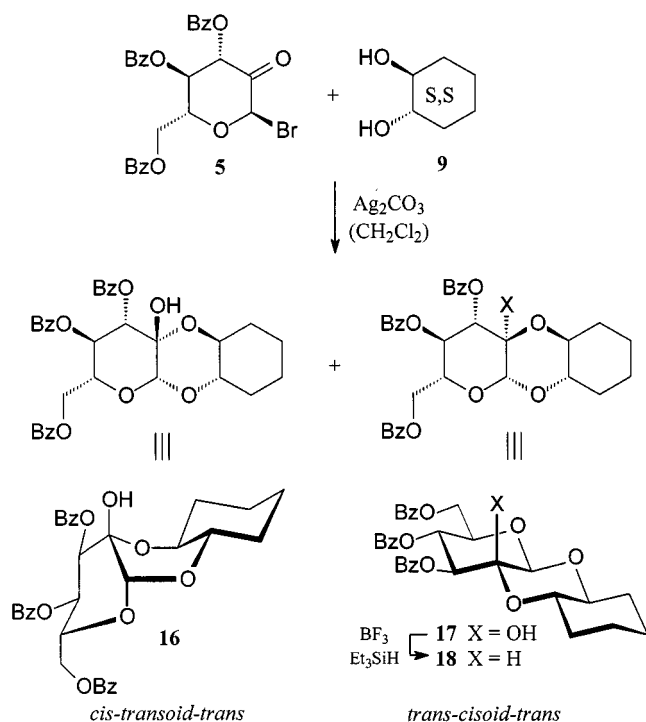
Scheme 4
